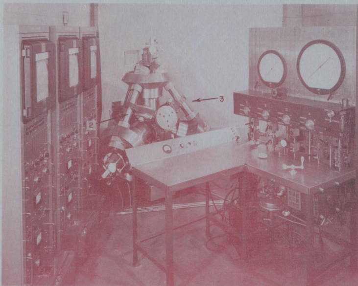
FIG. 1 COMPLETE TETRAHEDRAL-ANVIL HIGH PRESSURE, HIGH TEMPERATURE X-RAY DIFFRACTION APPARATUS
